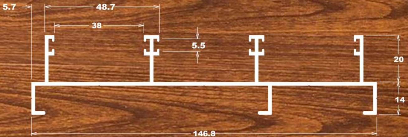
LG-064 1,728 Kg/m
