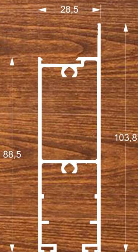
PR-32507 1,314 Kg/m
