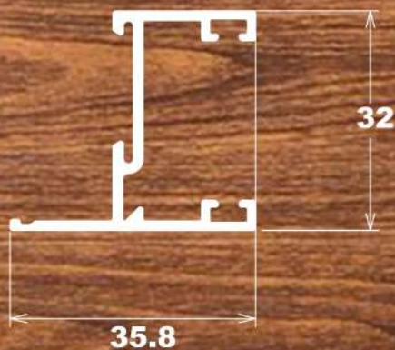
PR-32507 1,314 Kg/m
