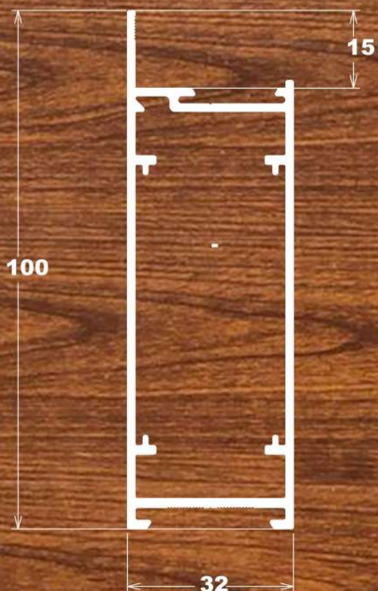
LG-042 1,169 Kg/m
