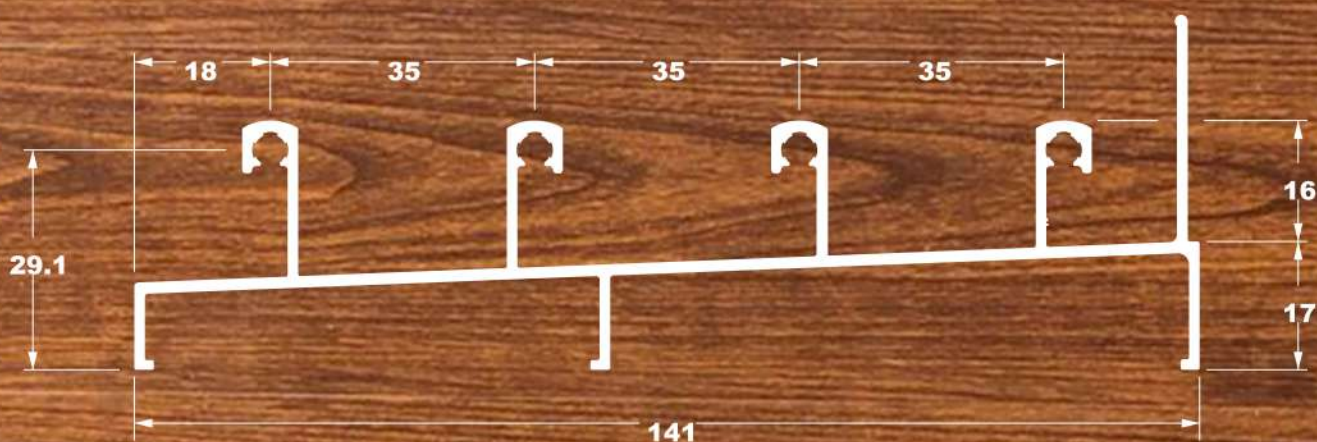
SU-122 1,512 Kg/m
