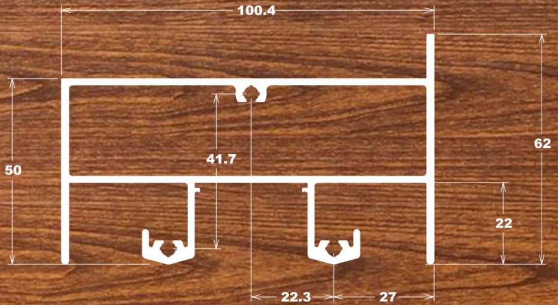
LG-005 2,134 Kg/m
