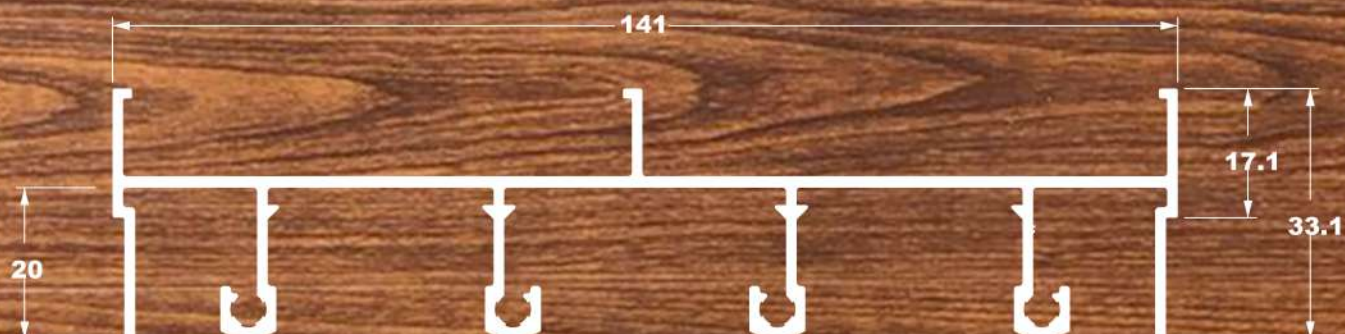
SU-121 1,586 Kg/m
